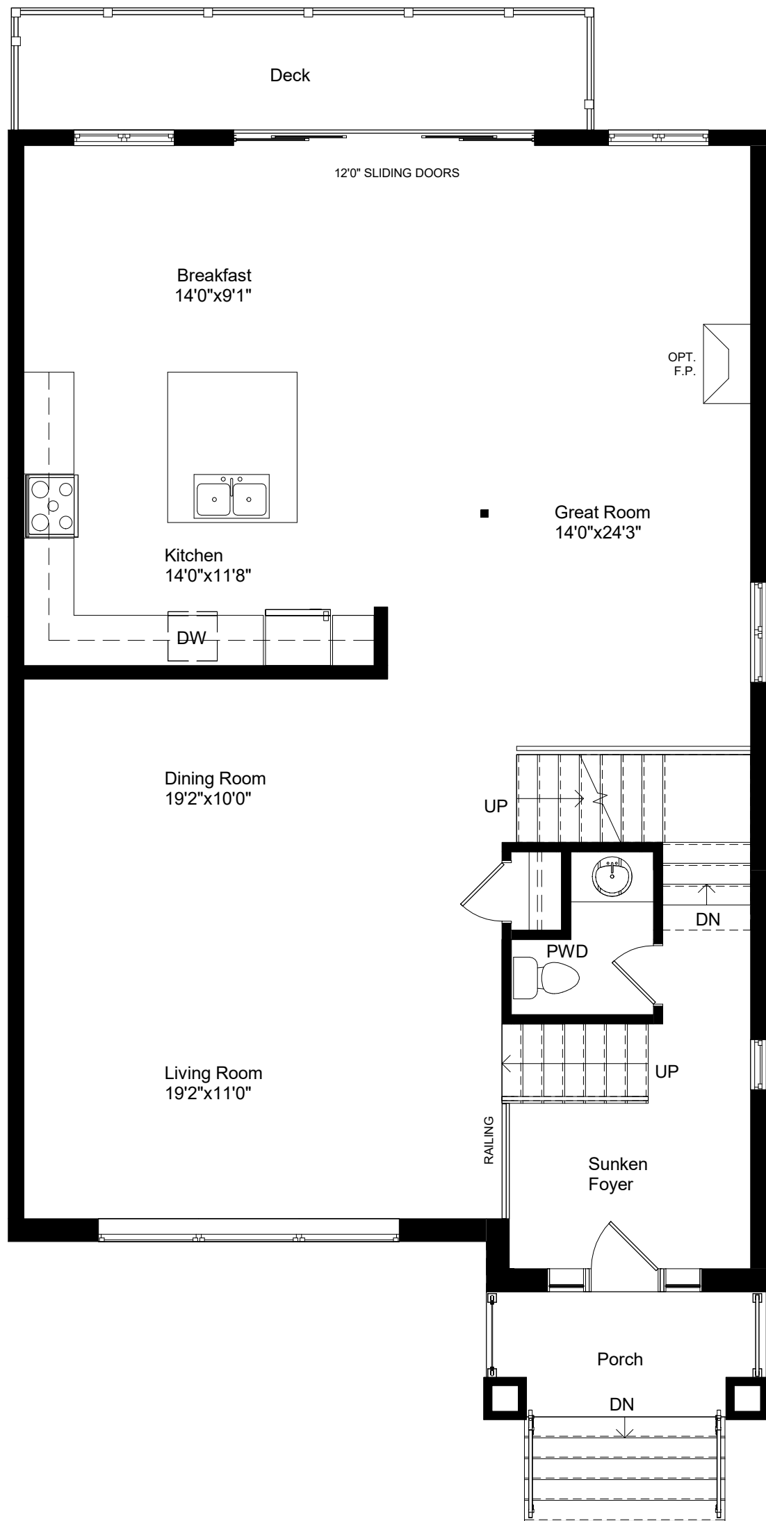
MAIN FLOOR PLAN OPTIONAL GREAT ROOM ENLARGED
